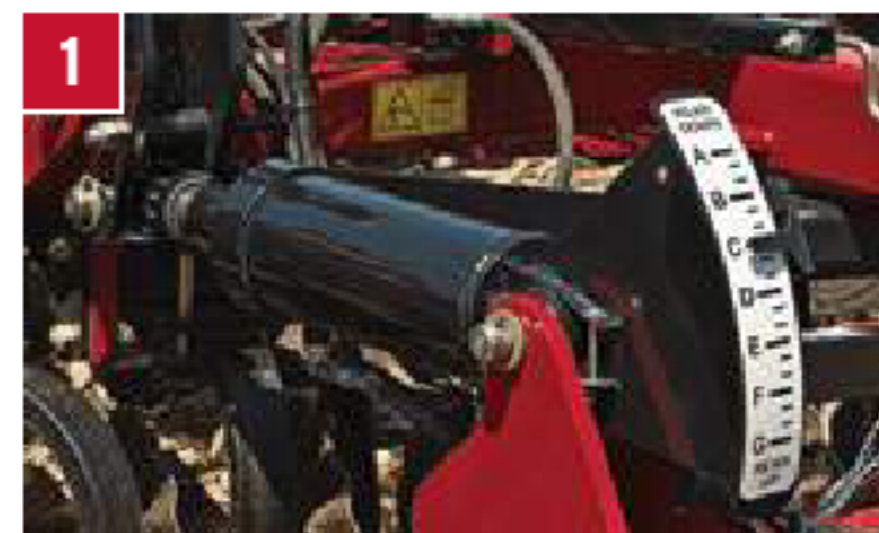
Hydraulic fore/aft control: maintain consistent agronomic output
