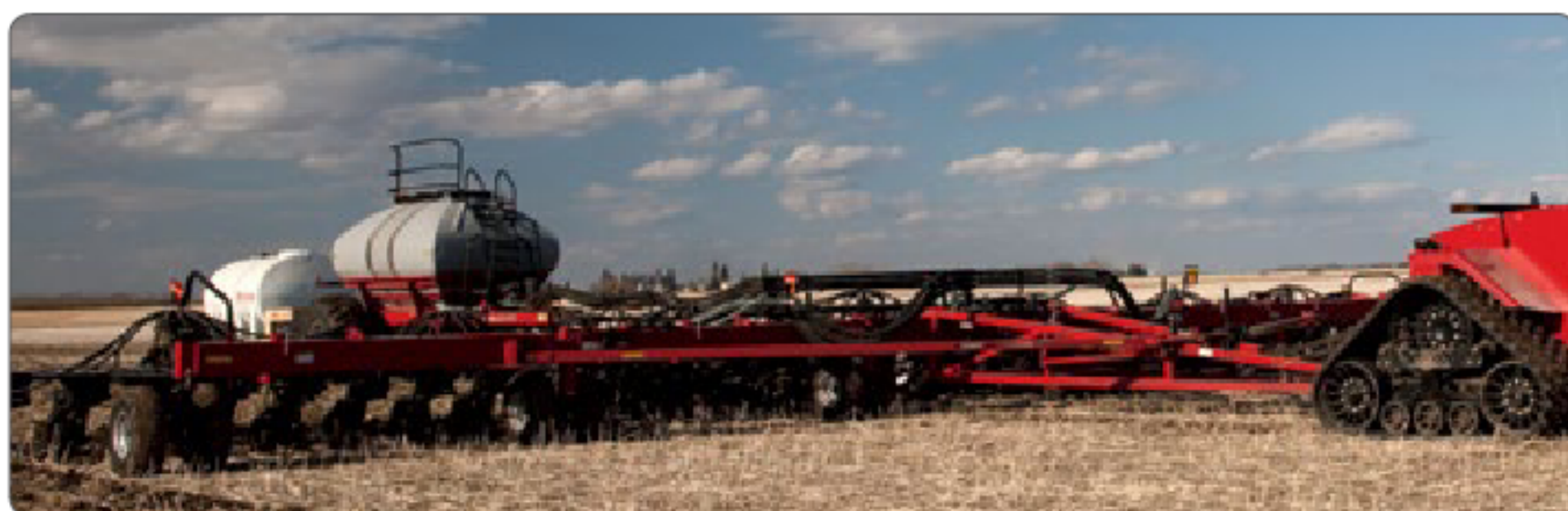
Case IH Precision Hoe™ air hoe drills deliver precise seed and fertilizer placement, making it ideal for seeding high-value, small-seed crops on large acreages. It combines precise control with rugged reliability thanks to the patented, parallel-link row unit and unique single-shank design that offers good residue flow in uneven terrain and tough no-till conditions.
