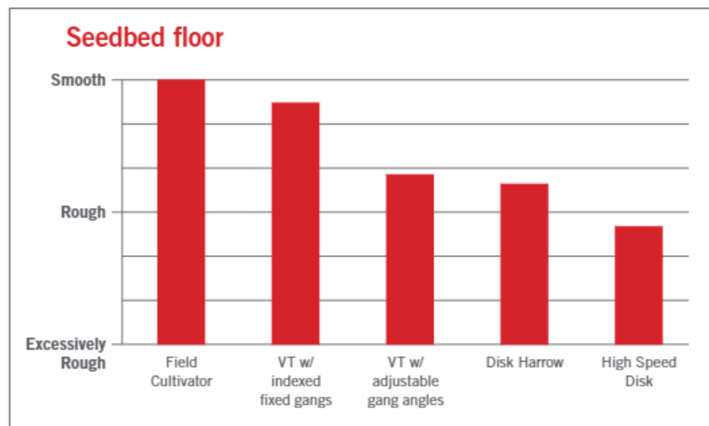
Seedbed floor quality for varying tillage tools
