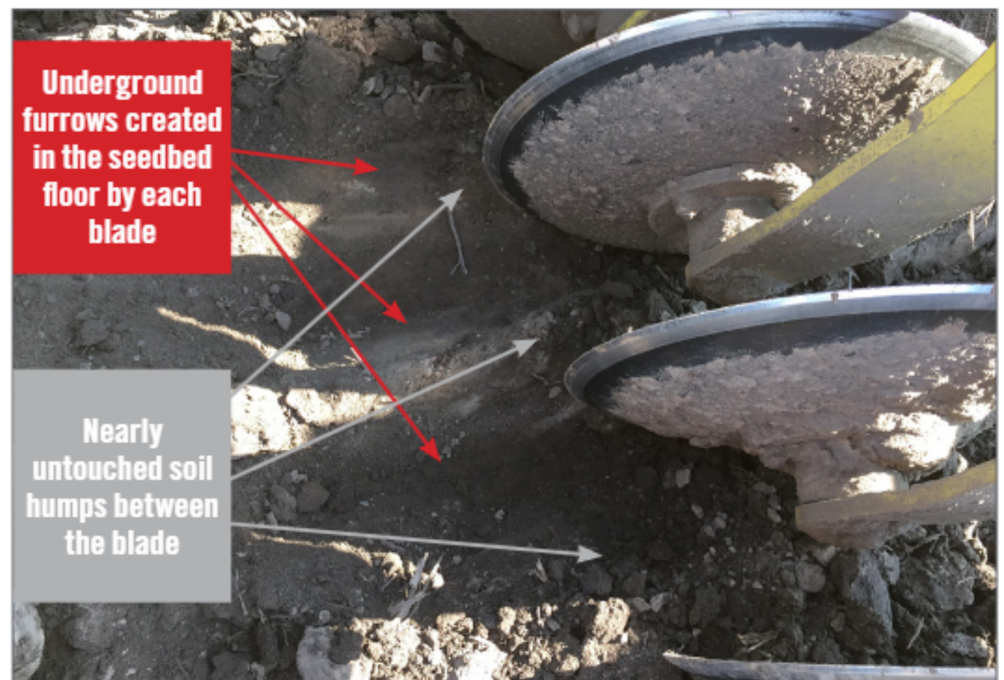
Seedbed floor created with high-speed disk
