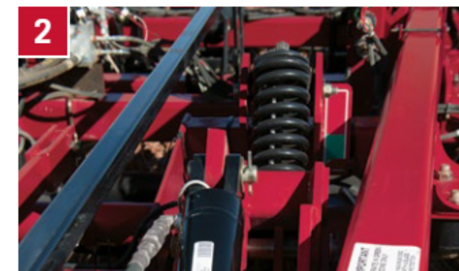
2 Disk gang pressure: reduce pressure on frame
