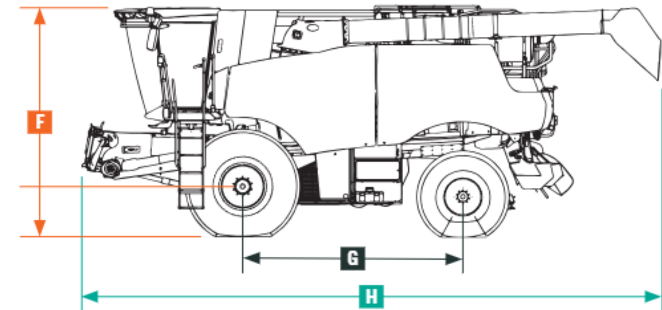
150 SERIES DIMENSIONS
