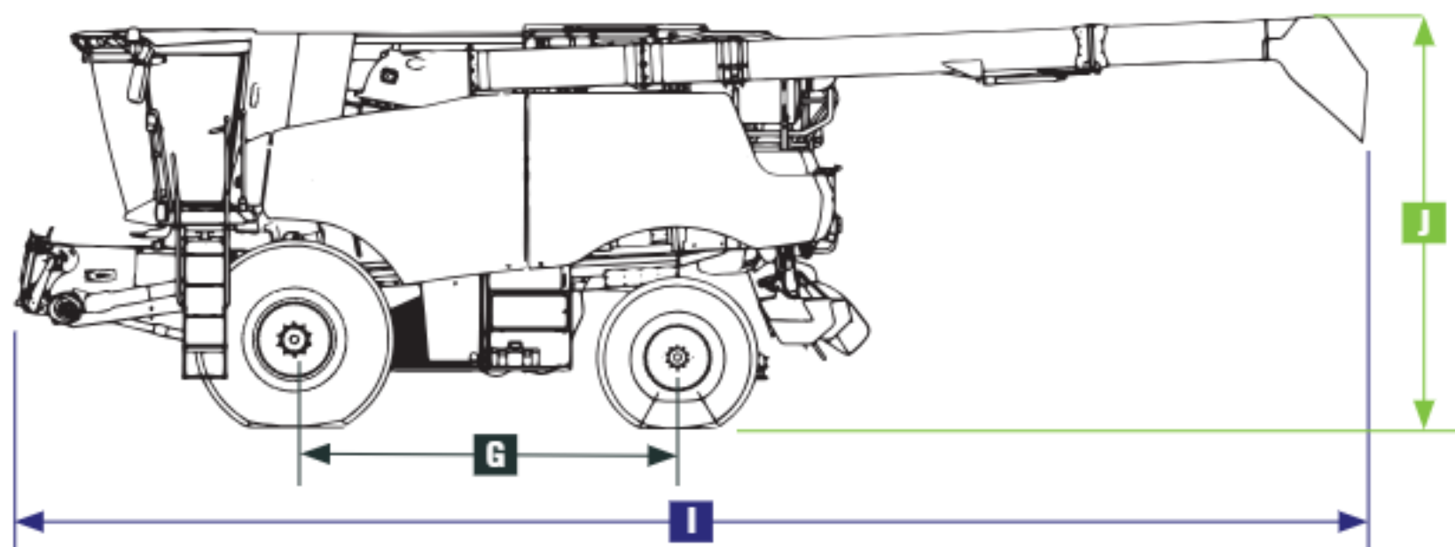
250 SERIES DIMENSIONS
