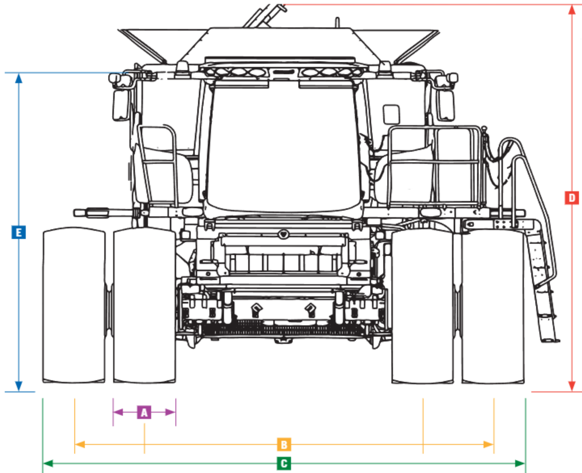
250 SERIES DIMENSIONS
