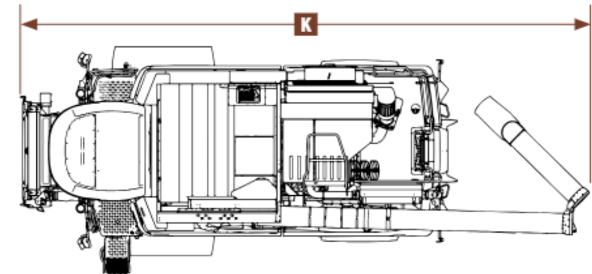
240 SERIES OVERALL LENGTH
