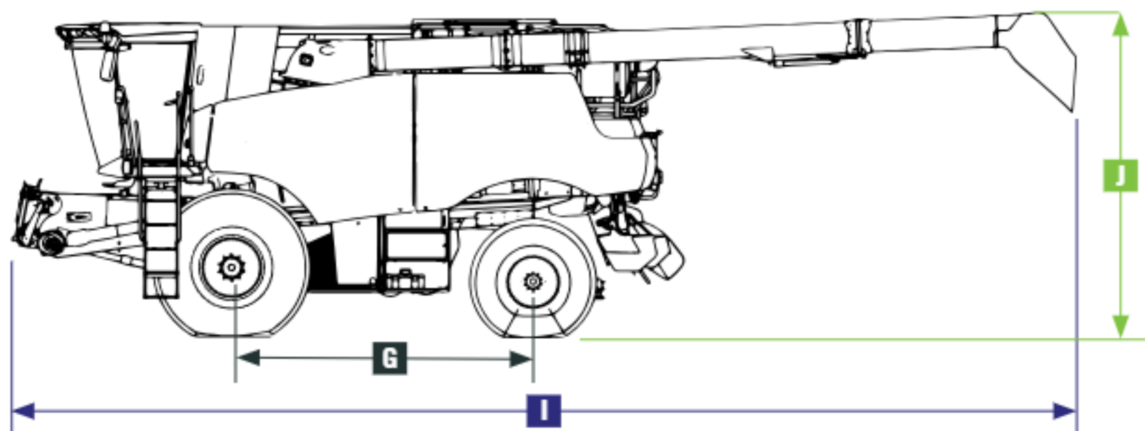
240 SERIES DIMENSIONS
