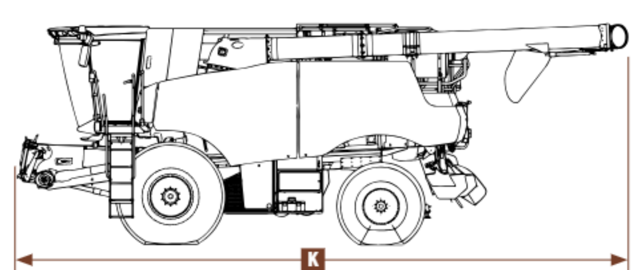
240 SERIES OVERALL LENGTH (AUGER FOLDED)
