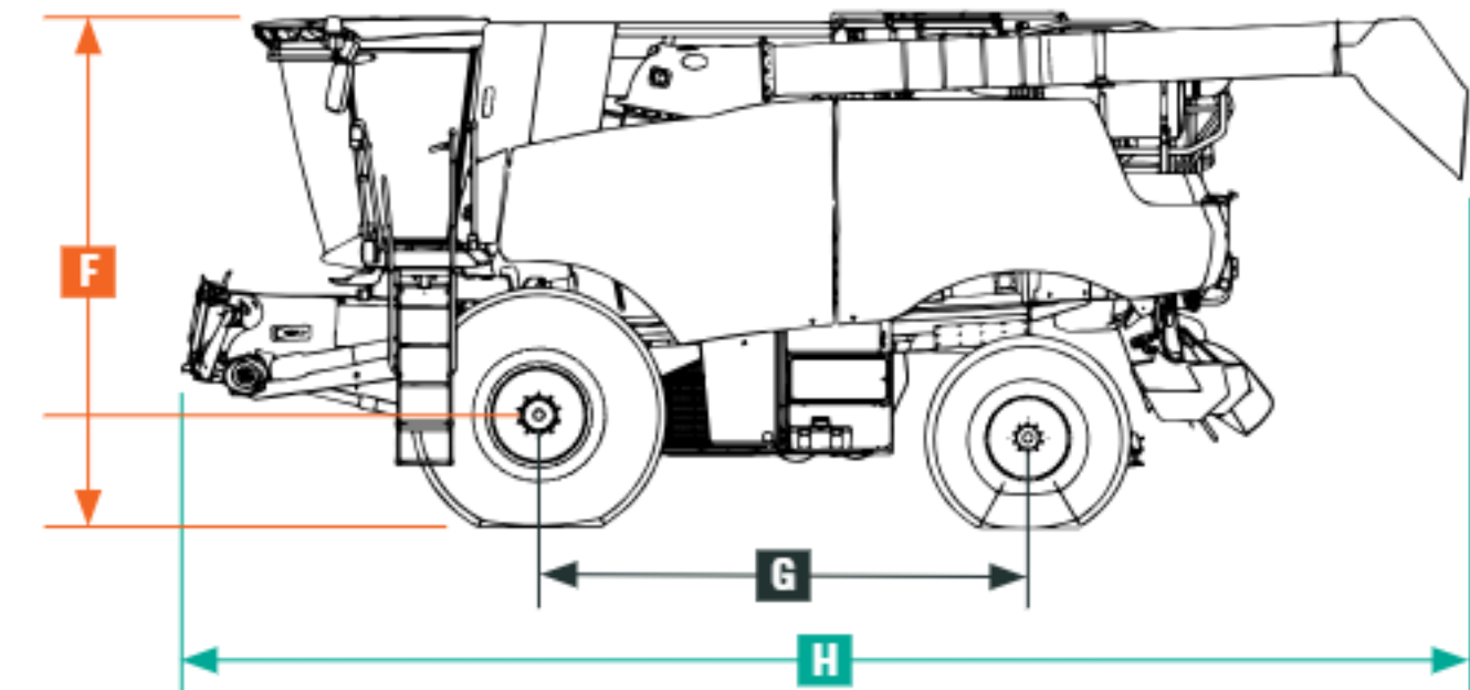
140 SERIES DIMENSIONS
