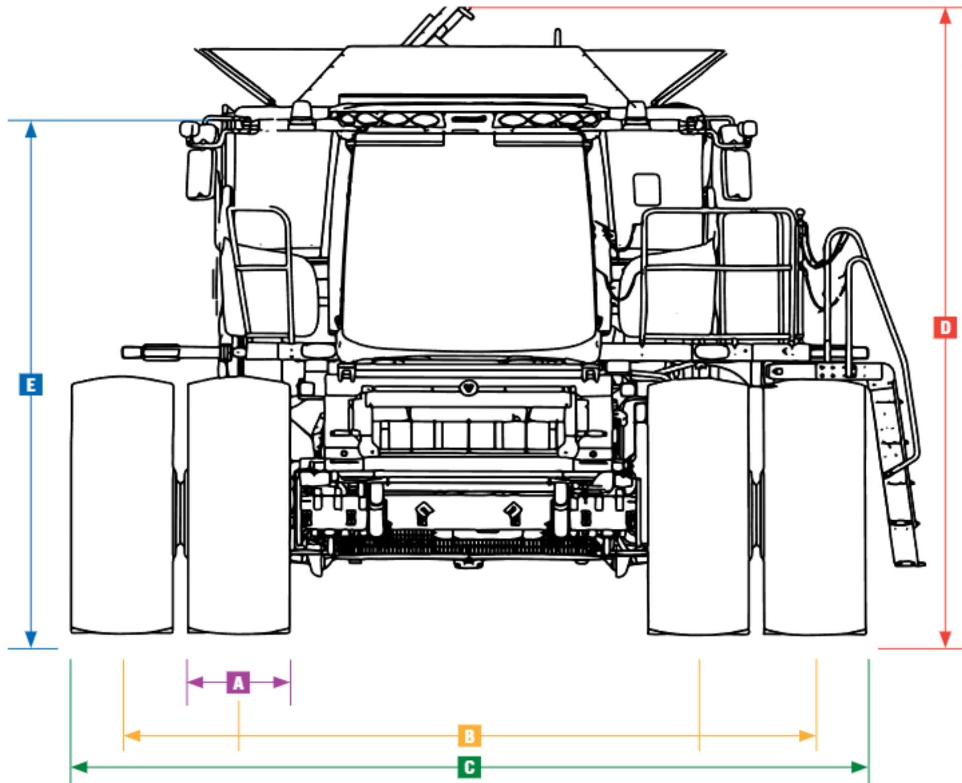
240 SERIES DIMENSIONS
